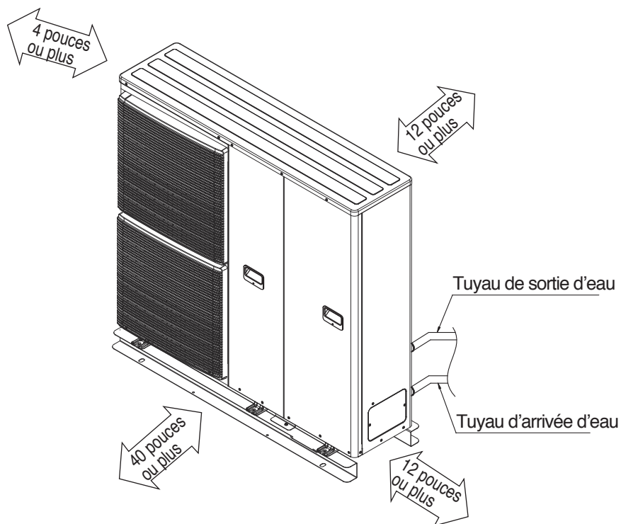
Figure 6-3 Distance minimale d'installation
